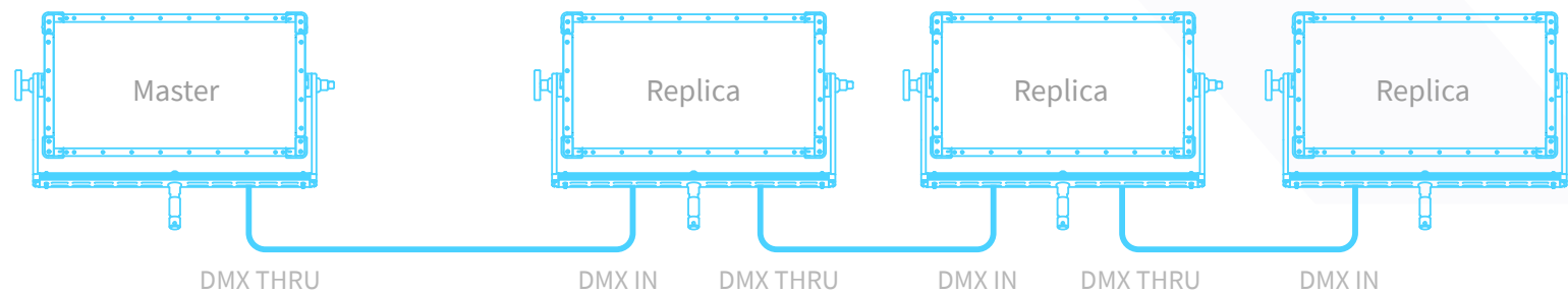
Replica Fixture
